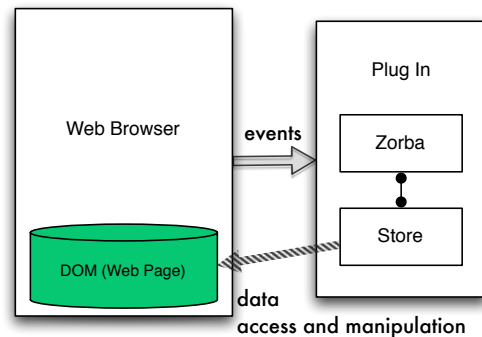
Figure 2: XQIB Architecture
