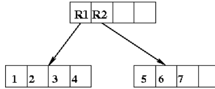
Figure 1: R-Tree with d=2
